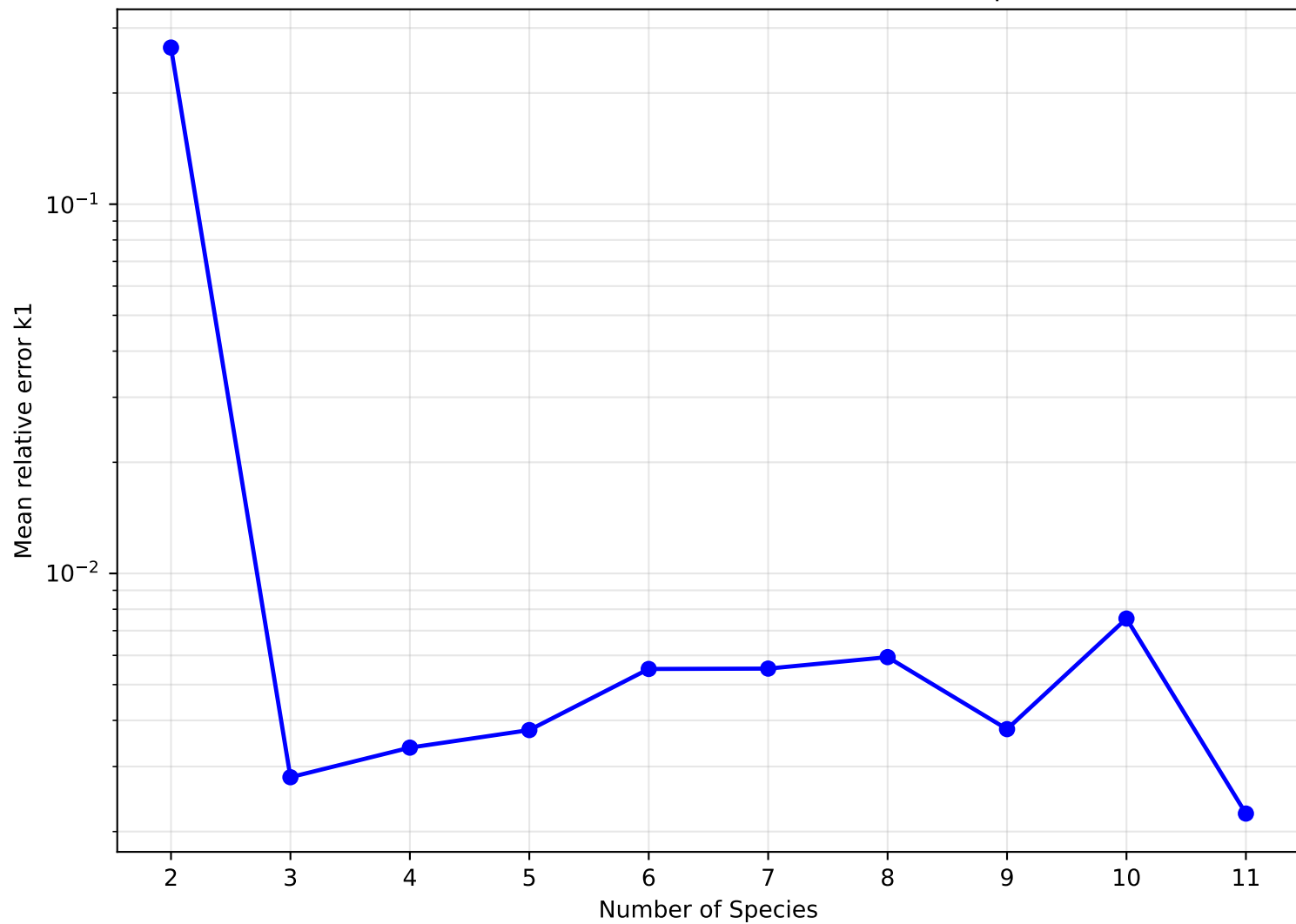
30, 30 — Mean relative error k1 vs number of species
